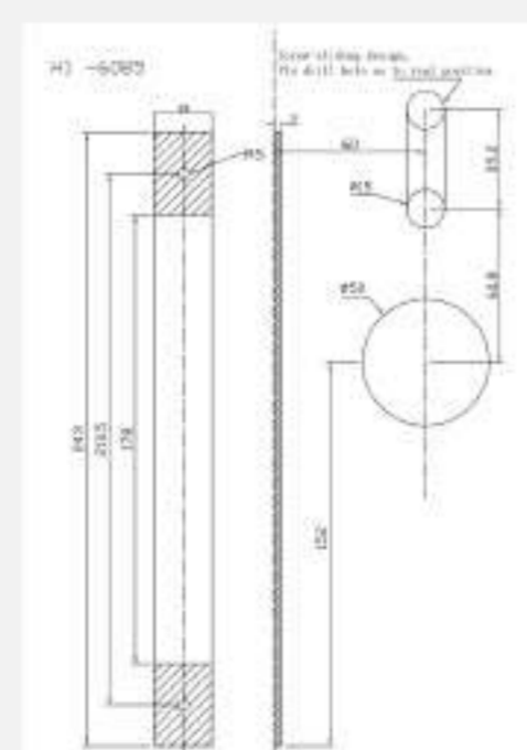
drilling template * 1
